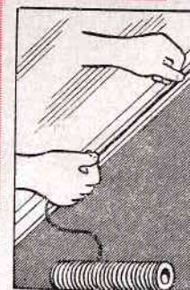
Applying (a) Sylglas Cord and (b) Sylglas Mastic into glazing bar rebates.
